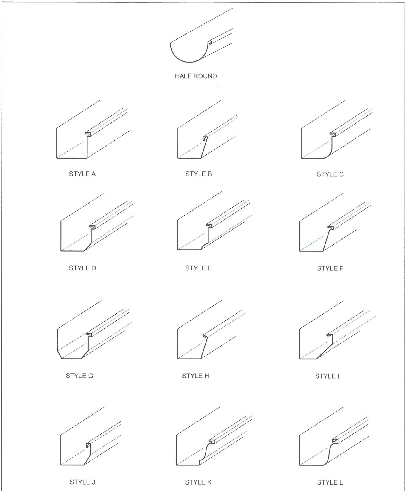
Figure 60: Examples of common gutter profiles
